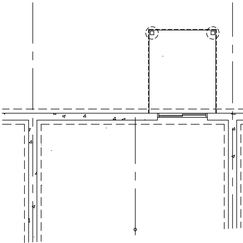
ALTERNATE WALK-OUT BASEMENT DETAIL
