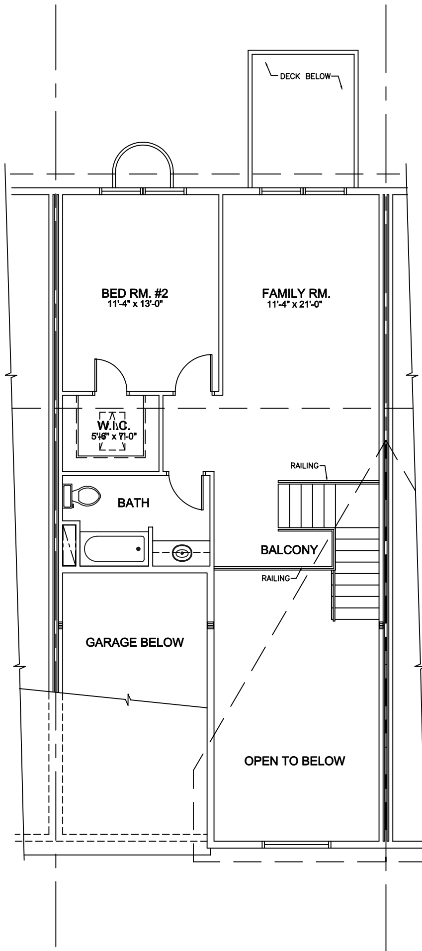
SECOND FLOOR PLAN (IN-LINE UNIT) 932 SQ. FT. (PER UNIT) SCALE: 1/4" = 1'-0"
