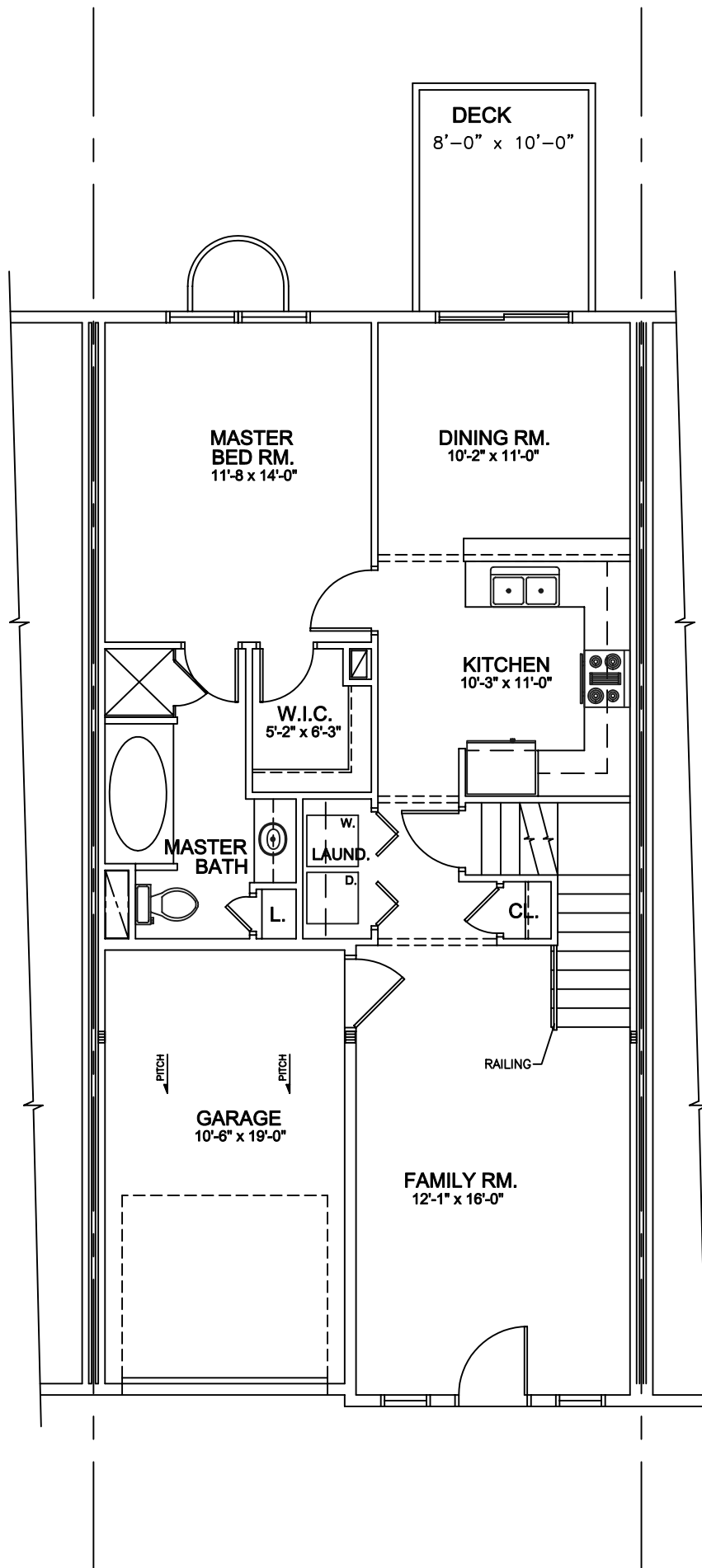
FIRST FLOOR PLAN (IN-LINE UNIT) 932 SQ. FT. (PER UNIT) SCALE: 1/4" = 1'-0" GARAGE: 215 SQ. FT. (PER UNIT)
